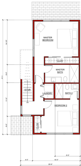
UPPER FLOOR
