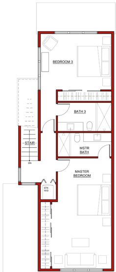
UPPER FLOOR
