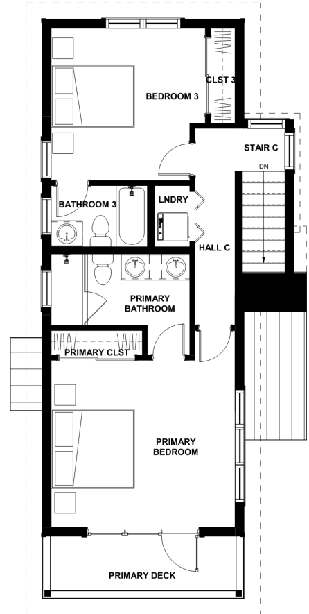
4 UPPER LEVEL - MRKG A2.4 1/4" = 1'-0"
