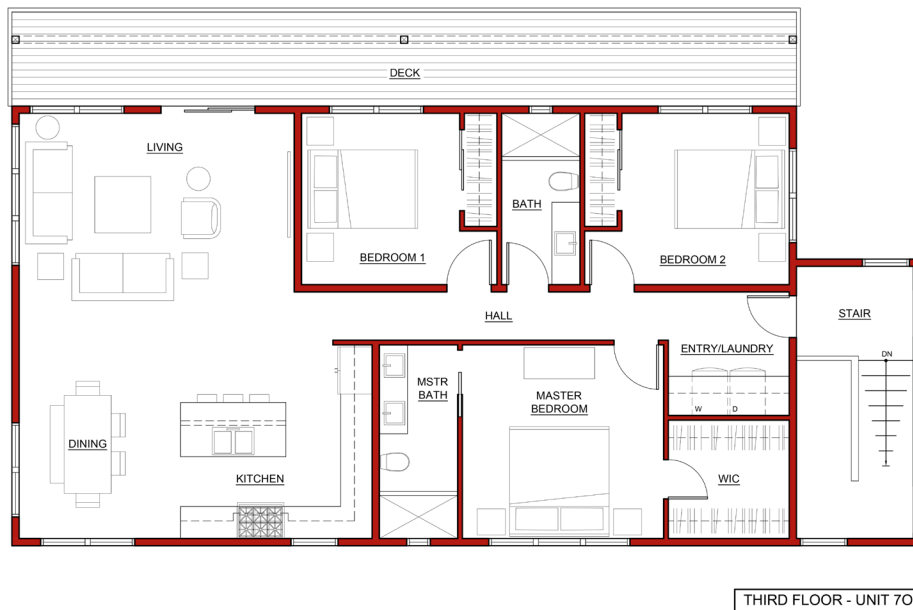
THIRD FLOOR - UNIT 70
